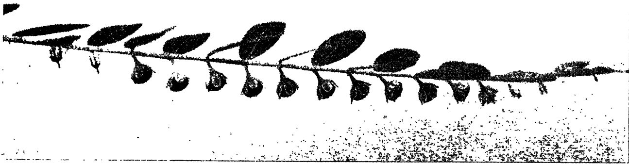
Plate 3.2 Developmental stages of the fruits of as seen from the Phyllanthus debilis , at the ventral side of leafy branch
