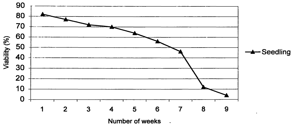
Figure 4.1 Viability variation of Phyllanthus debilis seeds for the period of nine weeks
