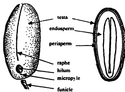
Plate 2.2 Morphology and anatomy of an typical seed
