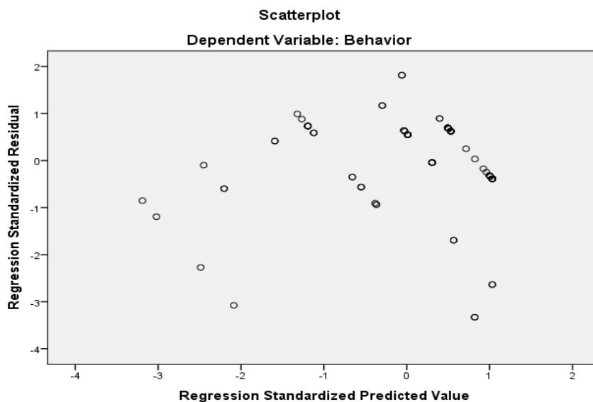
Figure 3 - Homoscedasticity
